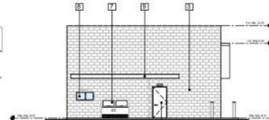
6 PROPOSED LEFT ELEVATION Scale: 1/8" = 1'-0"
