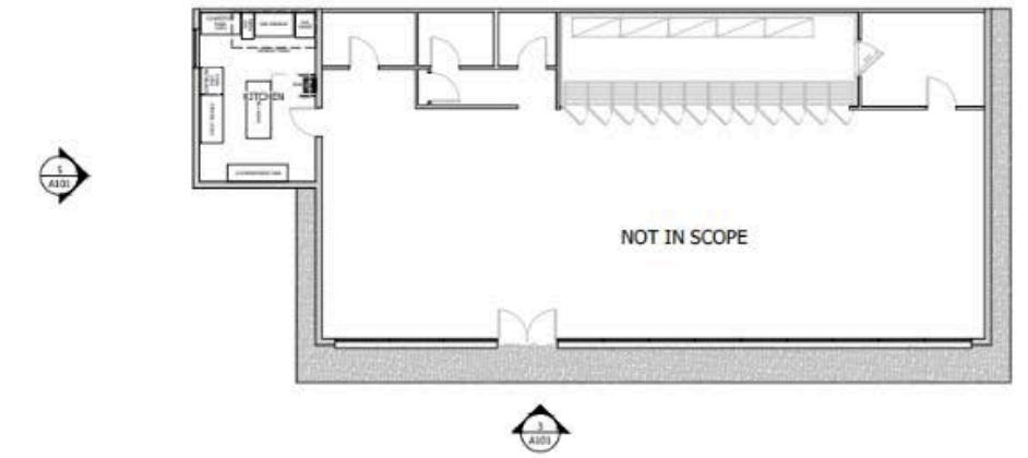
1 EXISTING FLOOR PLAN Scale: 1/8" = 1'-0"
